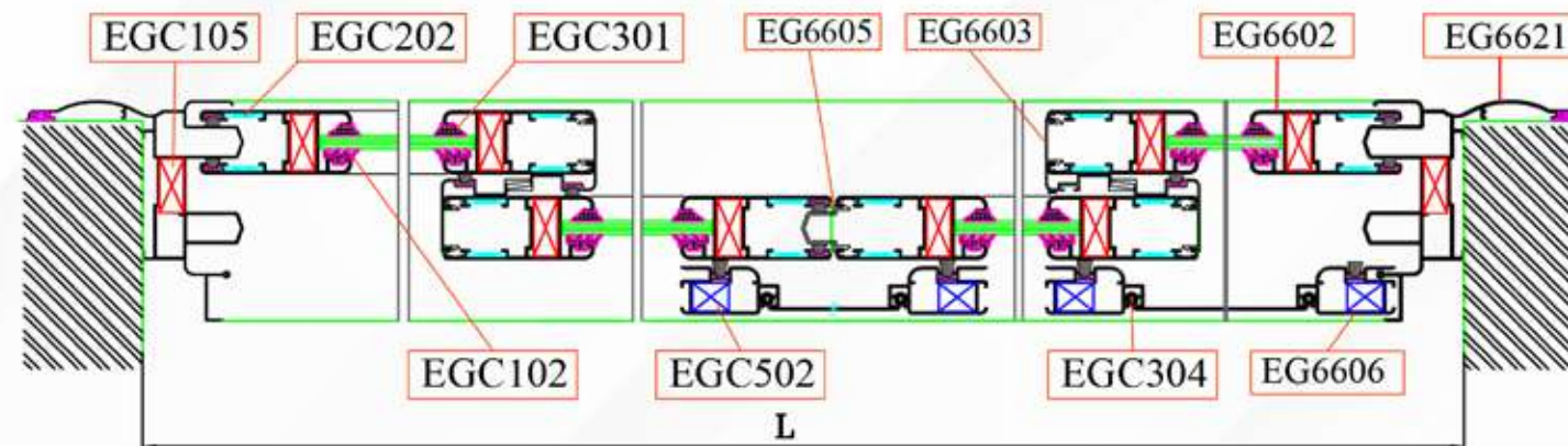
SECTION Z-Z
