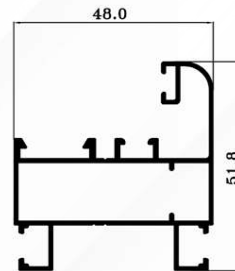
EG4800 0.855 Kg/ml.
