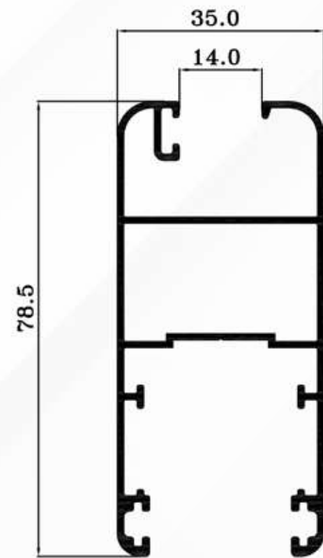
EG 9602 0.904 Kg/ml.
