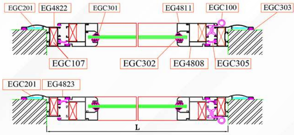
SECTION Z-Z
