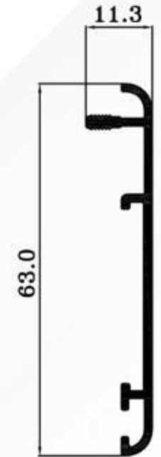
EG 5626 0.280 Kg/ml.
