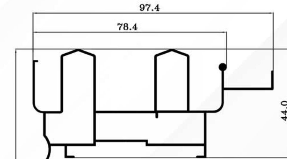
EG 6621 1.436 Kg/ml.
