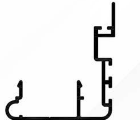
EG 9603 0.466 Kg/ml.
