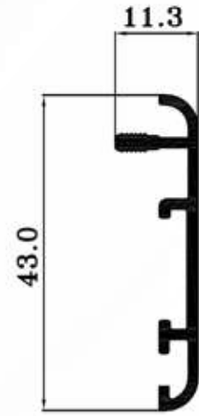
EG 5625 0.281 Kg/ml.
