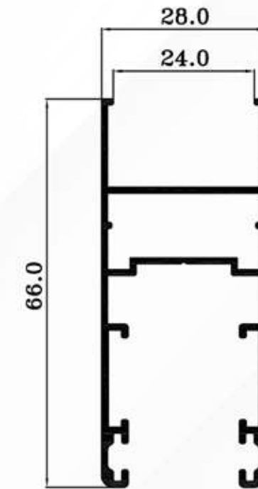
EG 6607 0.696 Kg/ml.
