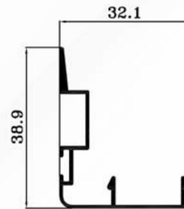
EG 6603 0.369 Kg/ml.
