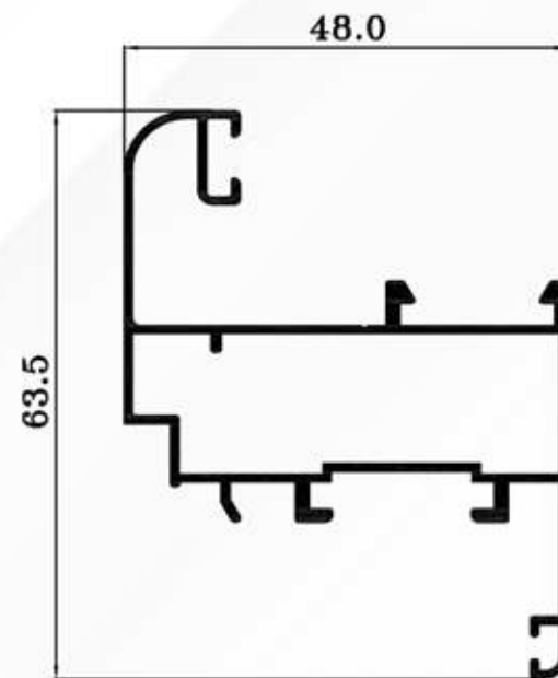
EG4807 0.850 Kg/ml.
