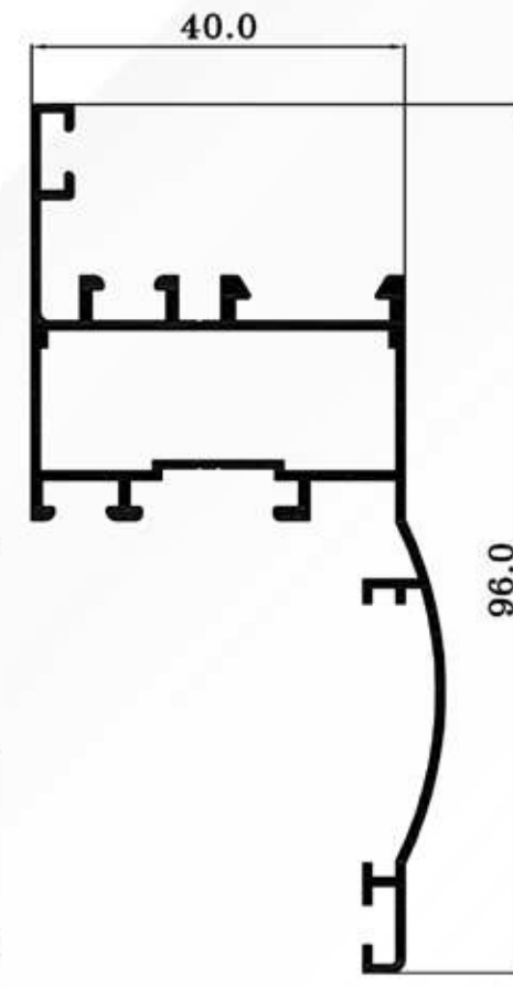
EG4822 0.970 Kg/ml.
