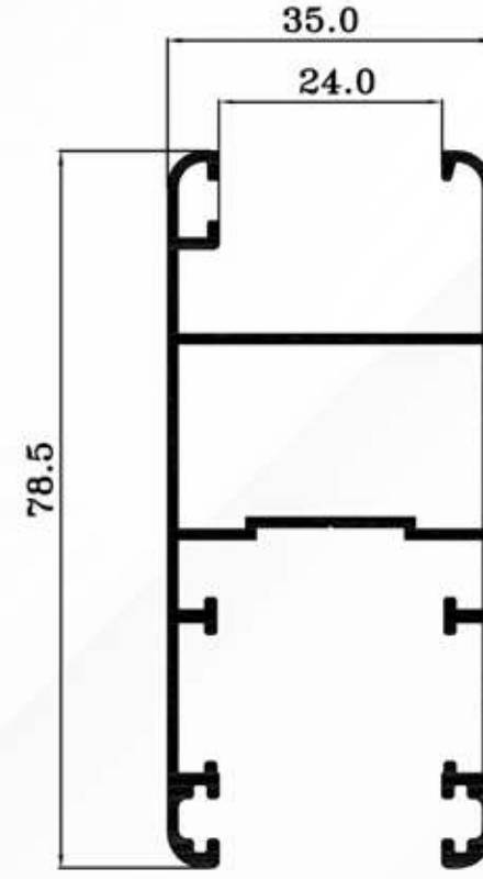
EG 9607 0.875 Kg/ml.
