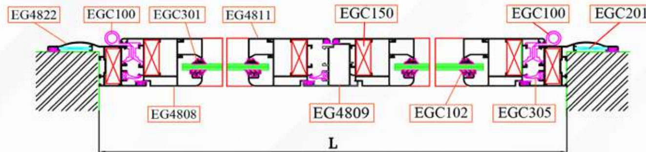
SECTION Z-Z
