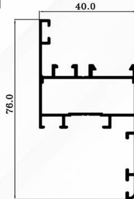
EG4801 0.840 Kg/ml.
