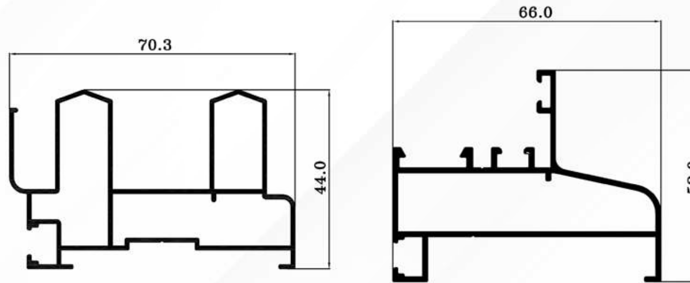
EG 6648 0.369 Kg/ml.
