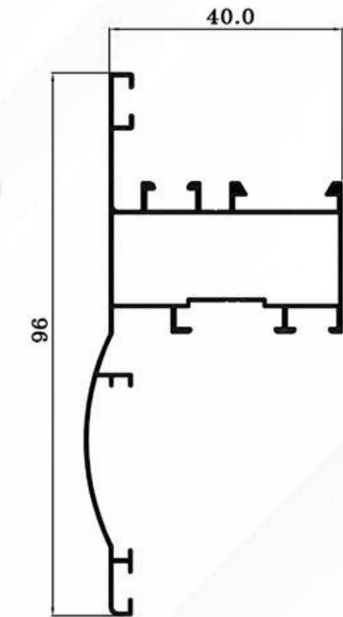
EG4823 0.970 Kg/ml.
